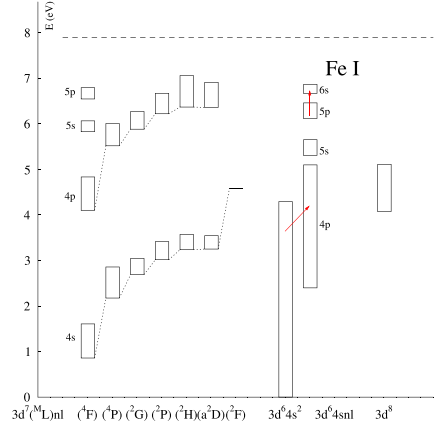
Figure 2. Energy level diagrams for Sc I and Fe I, respectively. The vertical energy scale is the same, and the dashed line shows the ionization energy. The observed lines are marked with red arrows. Note that the near-IR Sc I lines are located at significantly lower excitation energies compared to the near-IR Fe I lines.
