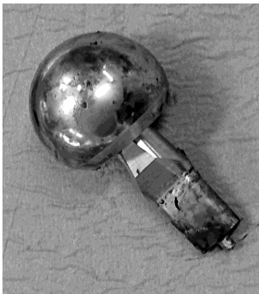
Figure 27: ABG II modular head (LFit) and neck after revision with corrosion on the neck part engaged in the stem/neck junction
