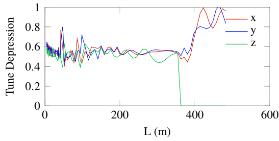
Figure 1: Tune depression in the ESS linac.
