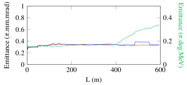
Figure 4: Emittance evolution in the ESS linac.
