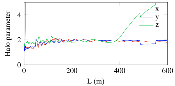
Figure 5: Halo parameter evolution in the ESS linac.
