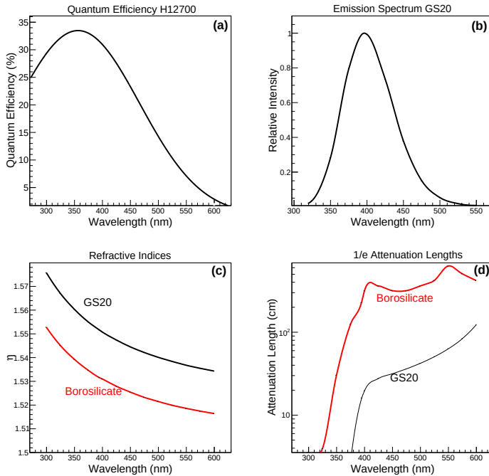
Figure 3: Optical properties employed in the simulation: (a) the quantum efficiency of the bialkalai cathode of the H12700 PMT [9], (b) the scintillation emission spectrum of GS20 [21], (c) refractive indices of GS20 [21] and borosilicate glass [22], (d) 1/e attenuation lengths of GS20 [21] and borosilicate glass [22].
