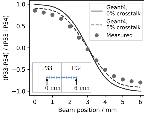
Figure 3.6: Light-sharing ratio formed from the Gaussian-fitted means of the pedestal- and gain-corrected charge distributions measured in P33 and P34 as the SoNDe module was scanned horizontally through a 1 mm FWHM thermal-neutron beam in 0.5 mm steps. The inset shows the irradiation positions. Uncertainties are smaller than the points and lines.
