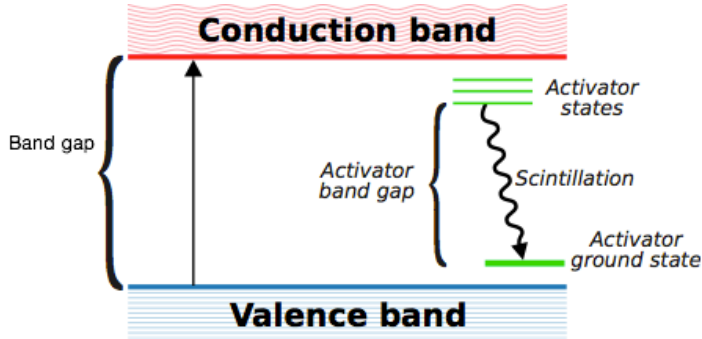
Figure 1.6: Electronic-band structure of an inorganic scintillator. Electrons in the valence band (blue) are excited to the conduction band (red) by the energy deposition of a particle in the scintillator. From the conduction band, the electrons de-excite via near-lying activator states (green) to the activator ground state by the emission of scintillation photons. Figure from [13], reproduced with the permission of the author.
