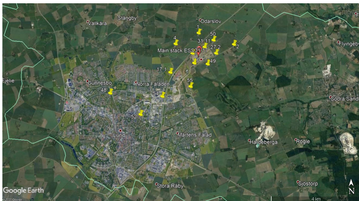
Figure 2. Sampling sites for ^{14}\text{C} samples for year 2018. See Table 3 for more information about the sampling sites.
