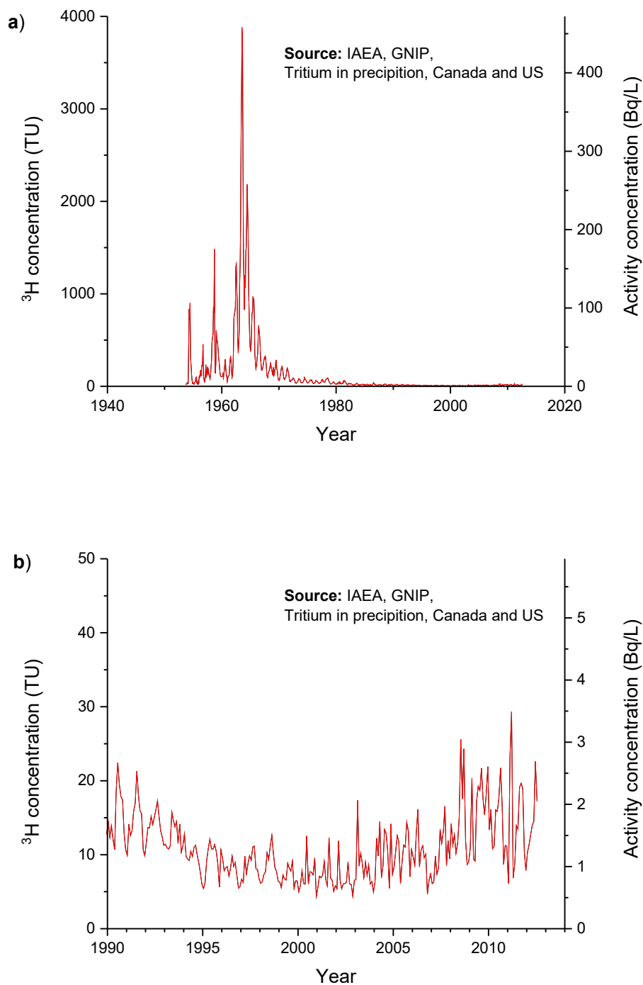
Figure 8 Tritium concentration in precipitation in Canada and the US [7] a) during the bomb-pulse era, b) from 1990 to 2012. 1 TU = 1 Tritium Unit, which equals 1 tritium atom per 10^{18} ^1\text{H} atoms, corresponding to 0.118 Bq/L of water.
