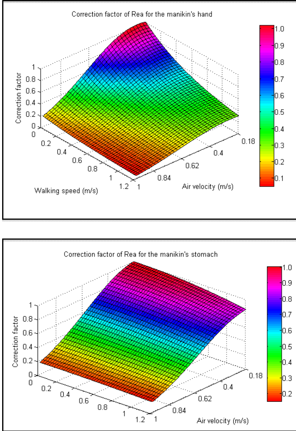
Fig 2. Correction/reduction factors of the boundary air layer's evaporative resistance ( R_{ea} ) for the manikin's right hand and stomach.
