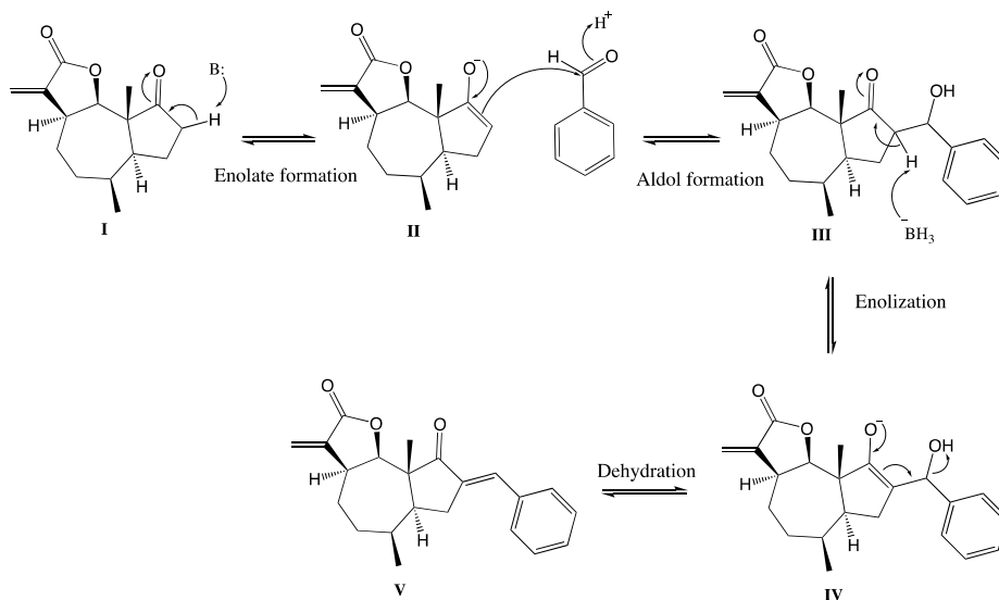
Figure 17. Mechanism of the Claisen-Schmidt base-catalyzed condensation between damsine and benzaldehyde.
