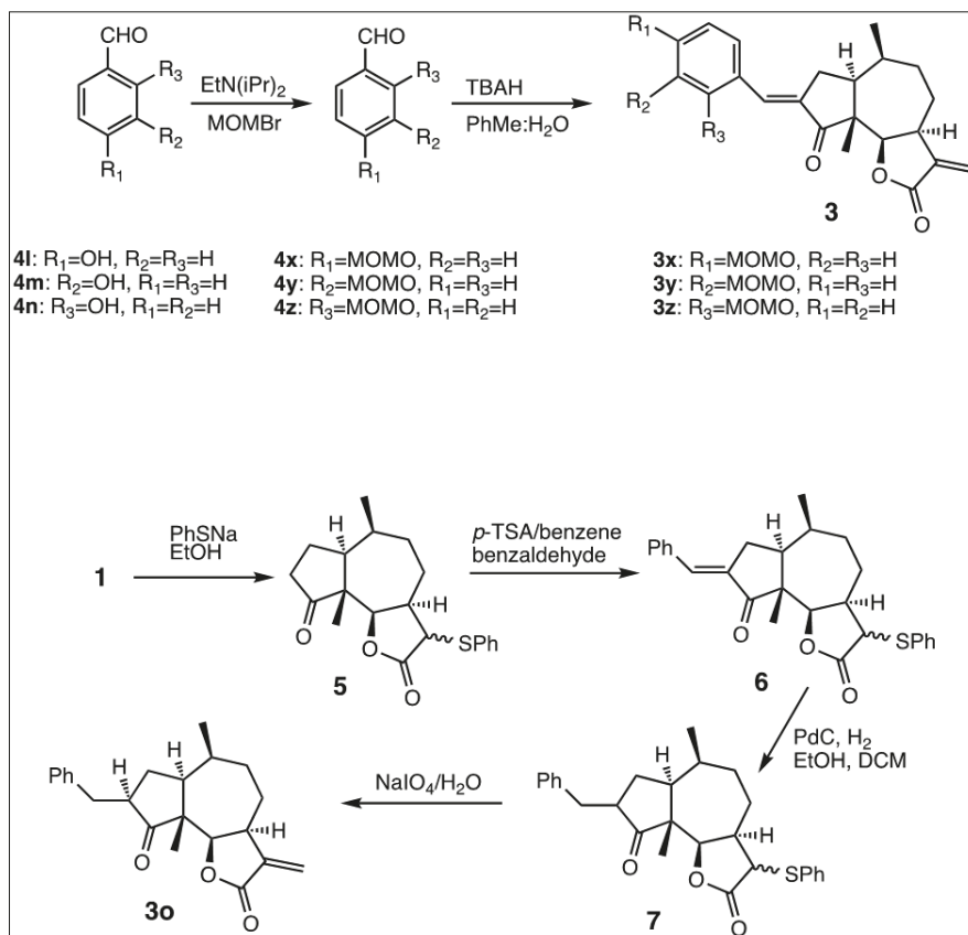
Figure 2. The hydroxybenzaldehydes 4l – 4n were protected using MOMBr and EtN(iPr)_2 , and the condensations of the protected hydroxybenzaldehydes 4x – 4z with 1 were carried out under basic conditions (3.2.1b). The reduced derivative 3o was prepared by protection of C-13 of 1 as a phenyl thiol ether ( 5 ), the condensation of 5 with benzaldehyde under acidic conditions (3.2.1a) to give 6 , which was hydrogenated to 7 and deprotected to yield 3o .
