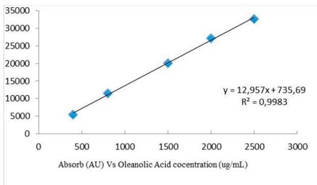
Figure N°2. Calibration curve of oleanolic acid
