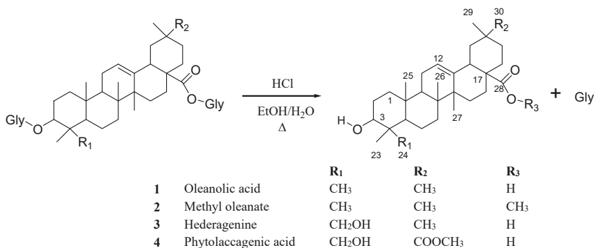
Figure 1. Acid hydrolysis of quinoa husks saponins to give four sapogenins
