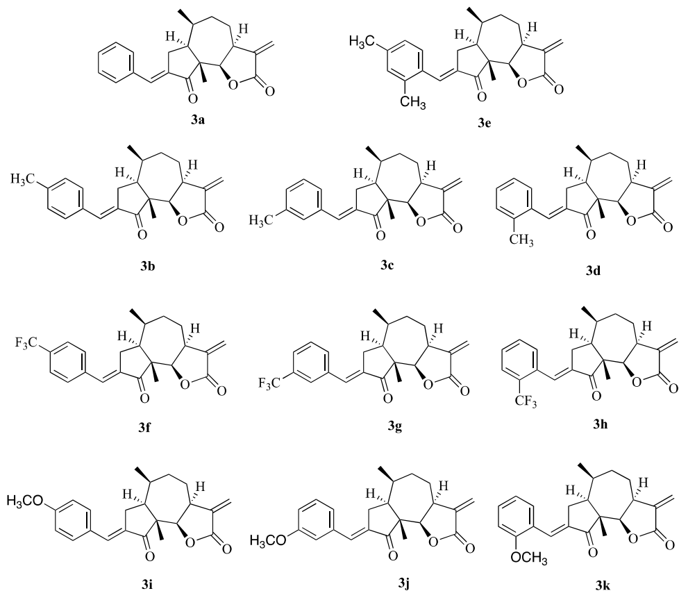
Figure 20. ( E )-3-(Benzyliden)damsin adducts from Claisen Schmidt condensation
