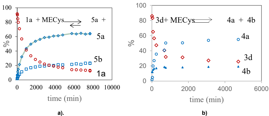
Figure 26. Kinetics of the Michael addition of a thiol to a) damsin 1a and b) benzylidene damsin derivative 3d
