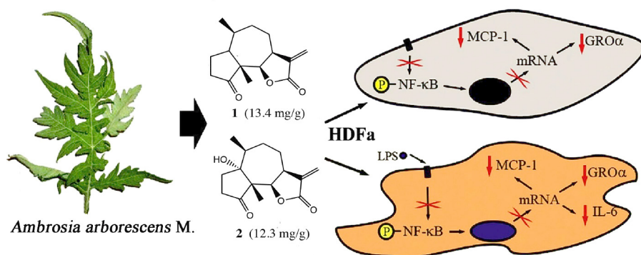
Figure 16. Damsin 1 and coronopilin 2 from A. arborescens 2, NF- \kappa B target genes involved in inflammation development
